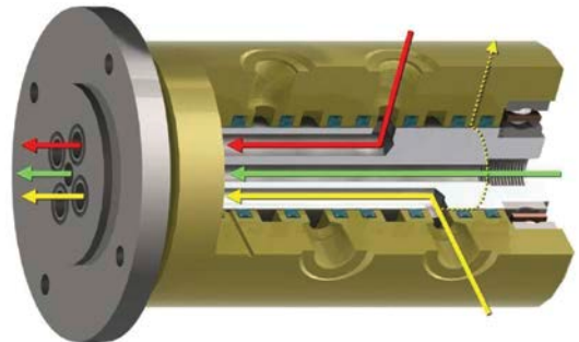
ROTATING UNION WITH PLASTOMERIC SEALS
