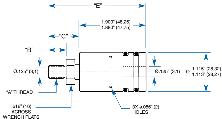
SHAFT MOUNTED Straight Model
